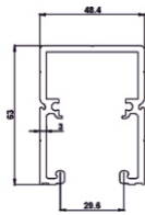
SST-024 Carrier Track
