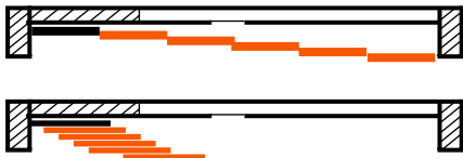
5 MOVING DOOR SLIDING SYSTEM SWSF 022-5
